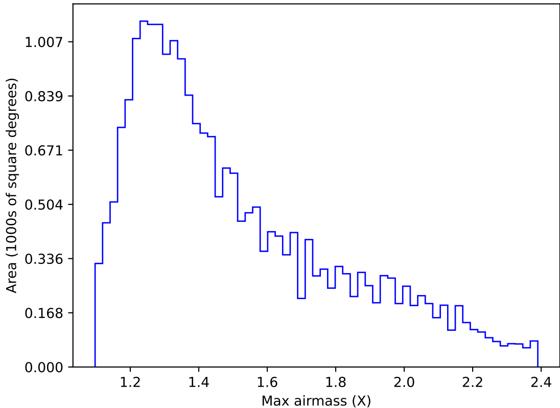
too_elab_heavy_r64_d3_gz_v3.4_10yrs Yr 1 u band: Max airmass
