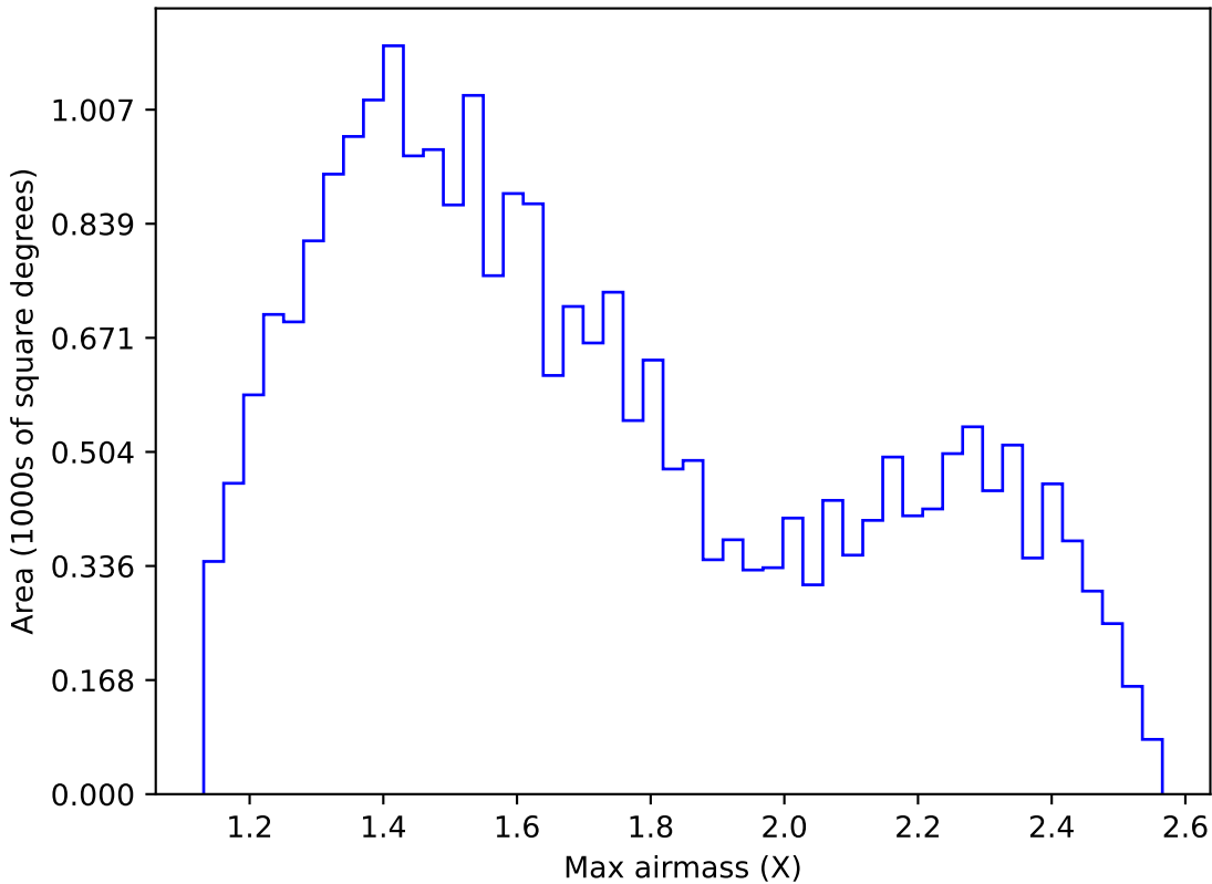
too_elab_heavy_r64_d3_gz_v3.4_10yrs Yr 1 r band: Max airmass
