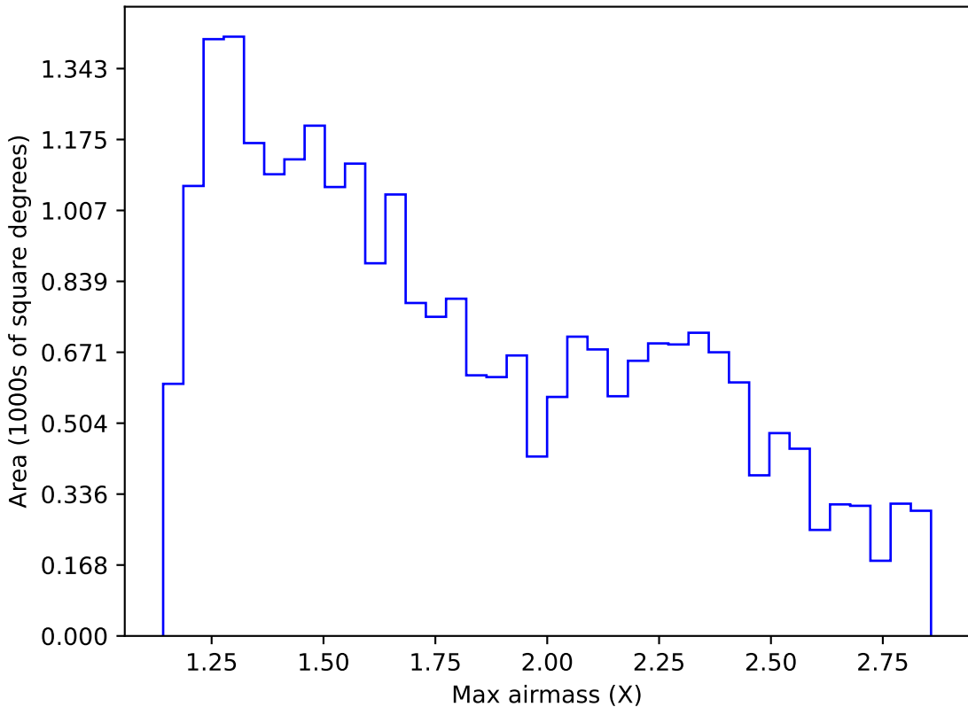
too_elab_heavy_r64_d3_gz_v3.4_10yrs Yr 1 i band: Max airmass
