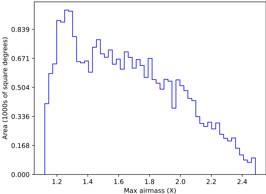
too_elab_heavy_r64_d3_gz_v3.4_10yrs Yr 1 g band: Max airmass
