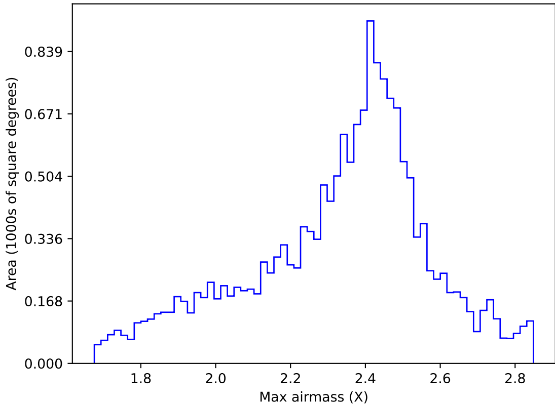
too_elab_heavy_r64_d3_gz_v3.4_10yrs WFD r band: Max airmass
