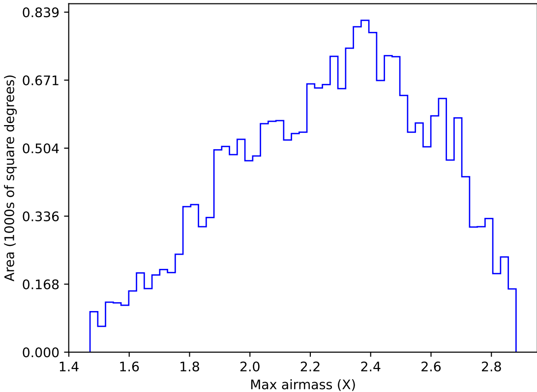
too_elab_heavy_r64_d3_gz_v3.4_10yrs All sky y band: Max airmass
