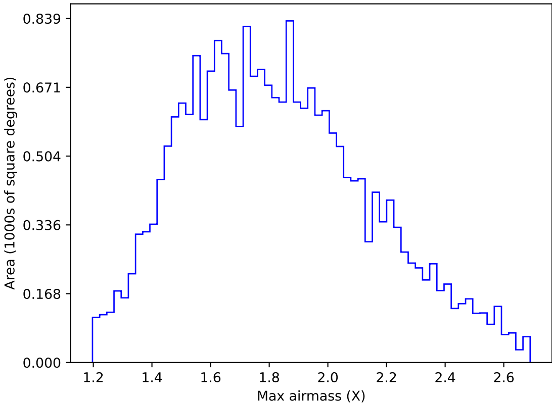
too_elab_heavy_r64_d3_gz_v3.4_10yrs All sky u band: Max airmass
