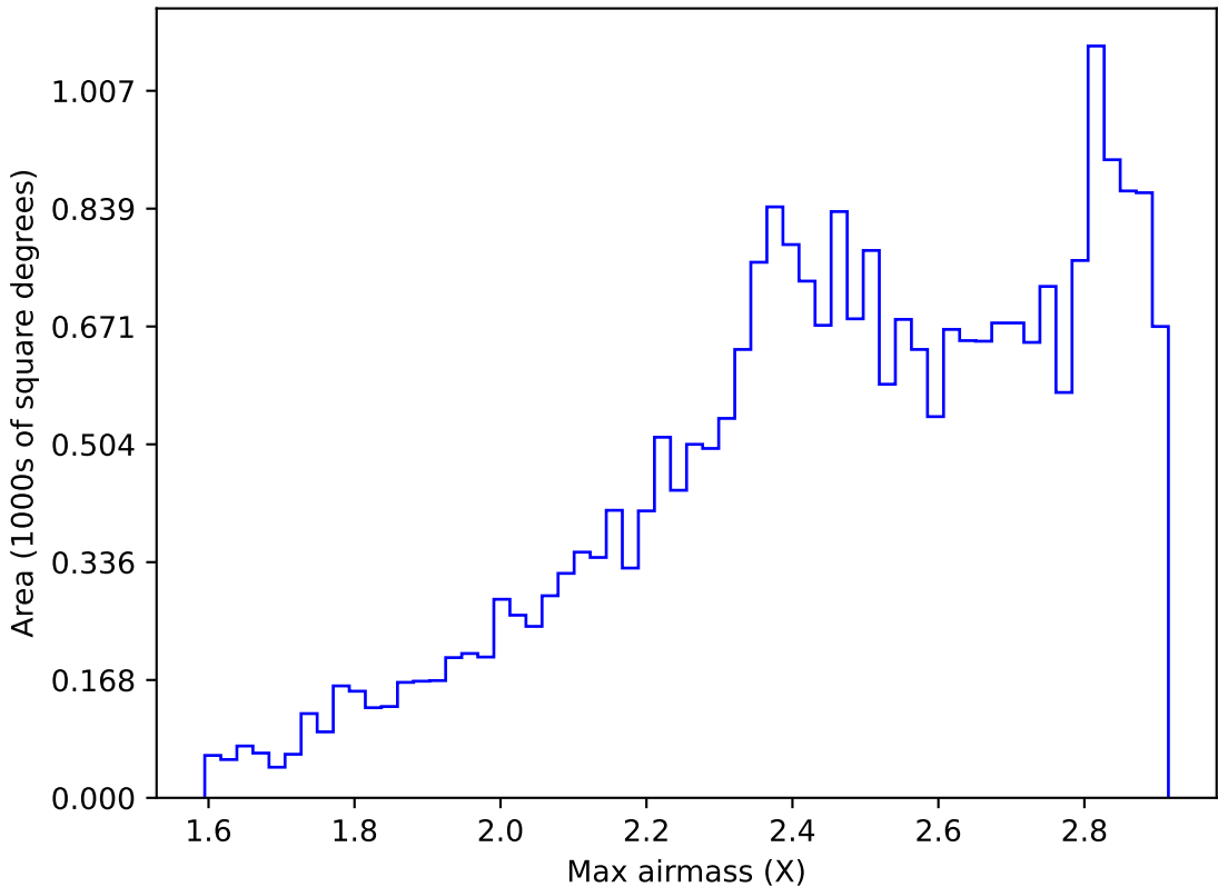
too_elab_heavy_r64_d3_gz_v3.4_10yrs All sky i band: Max airmass
