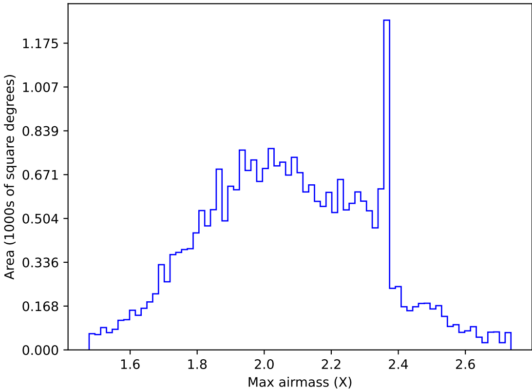
too_elab_heavy_r64_d3_gz_v3.4_10yrs All sky g band: Max airmass
