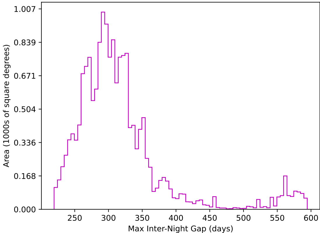
too_elab_heavy_r64_d3_gz_v3.4_10yrs WFD z band: Max Inter-Night Gap
