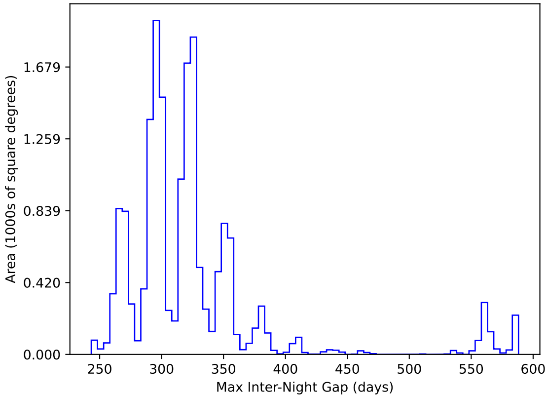
too_elab_heavy_r64_d3_gz_v3.4_10yrs WFD y band: Max Inter-Night Gap
