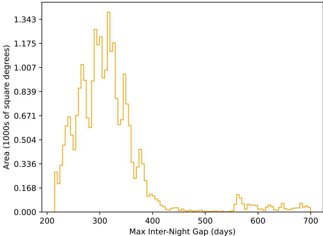
too_elab_heavy_r64_d3_gz_v3.4_10yrs All sky r band: Max Inter-Night Gap
