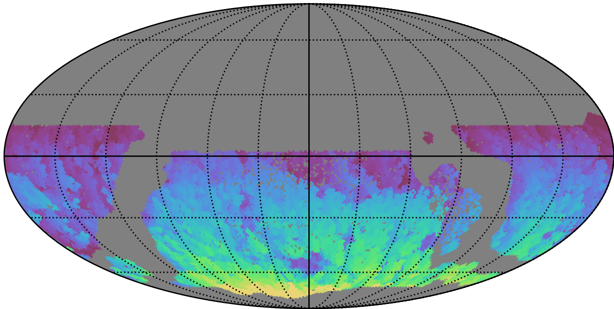
too_elab_heavy_r64_d3_gz_v3.4_10yrs WFD z band: Max HA
