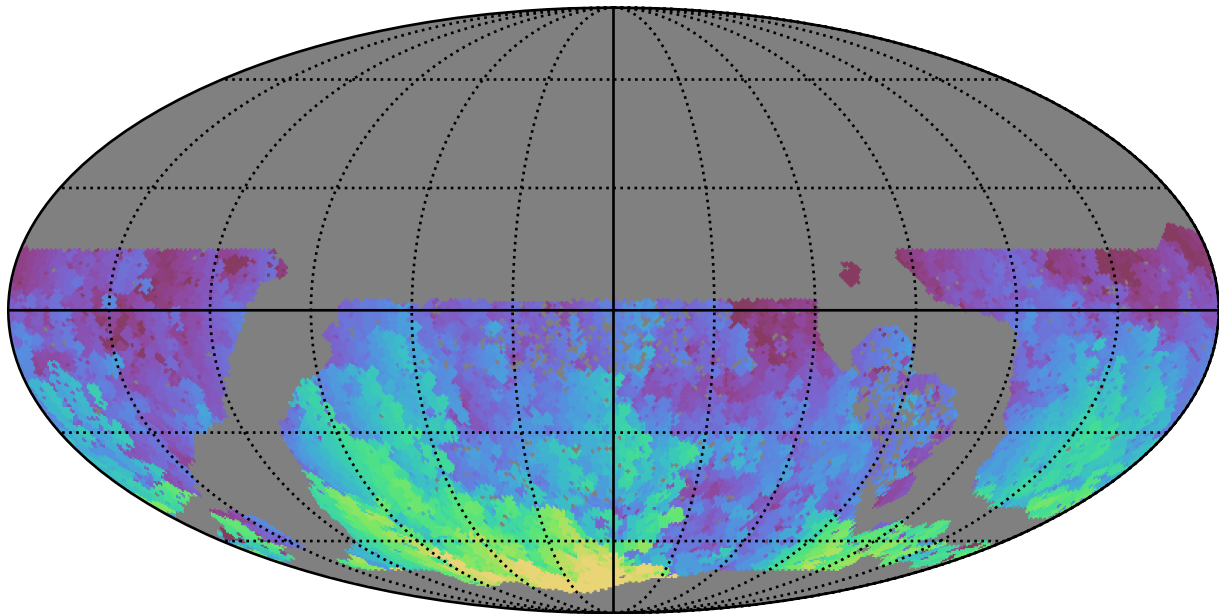
too_elab_heavy_r64_d3_gz_v3.4_10yrs WFD u band: Max HA
