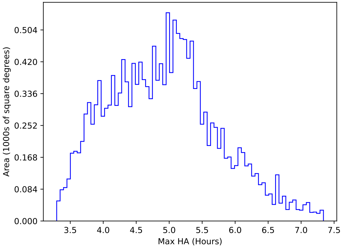
too_elab_heavy_r64_d3_gz_v3.4_10yrs WFD i band: Max HA
