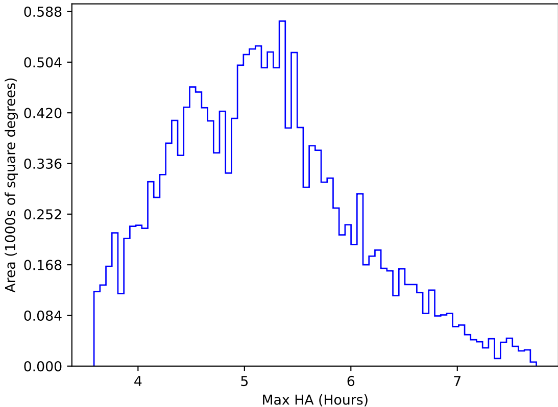
too_elab_heavy_r64_d3_gz_v3.4_10yrs WFD all bands: Max HA
