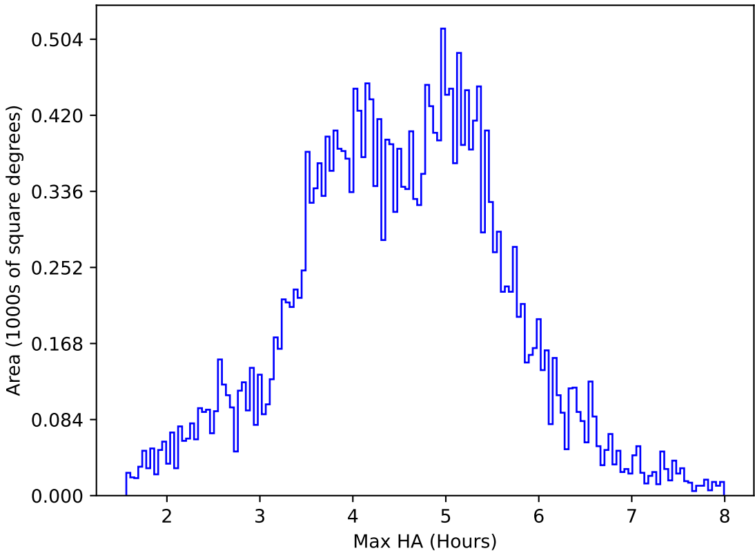
too_elab_heavy_r64_d3_gz_v3.4_10yrs All sky z band: Max HA
