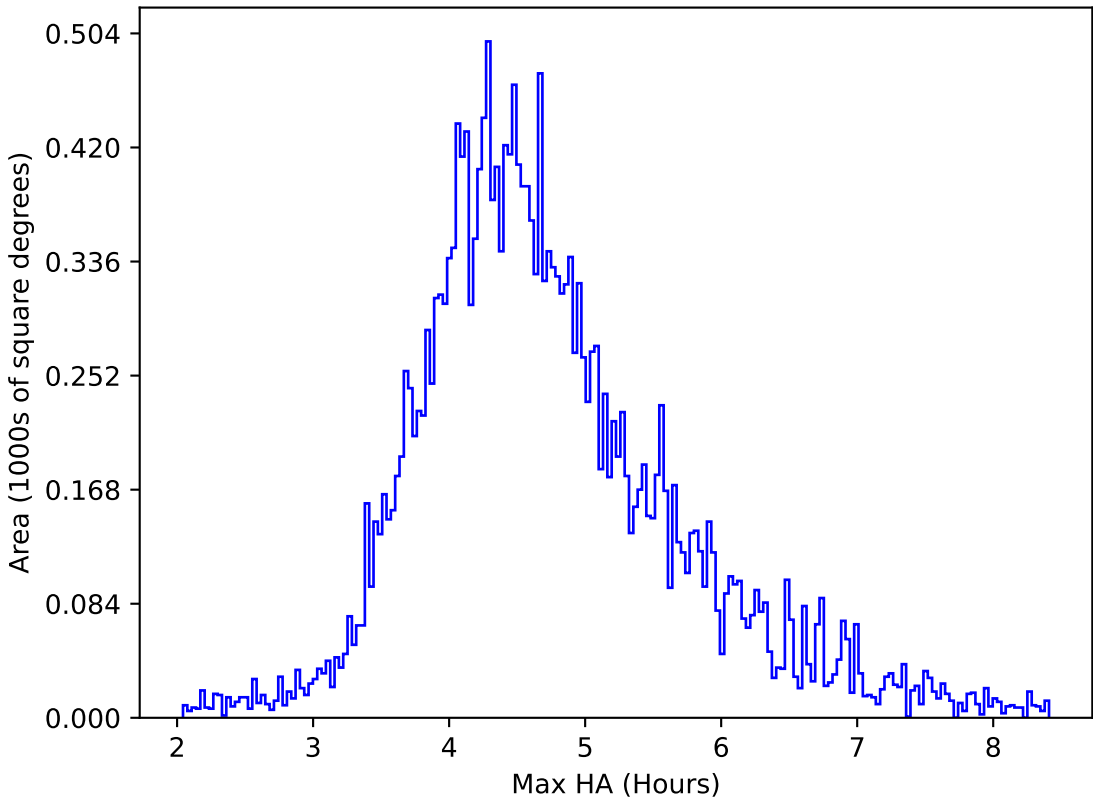
too_elab_heavy_r64_d3_gz_v3.4_10yrs All sky y band: Max HA
