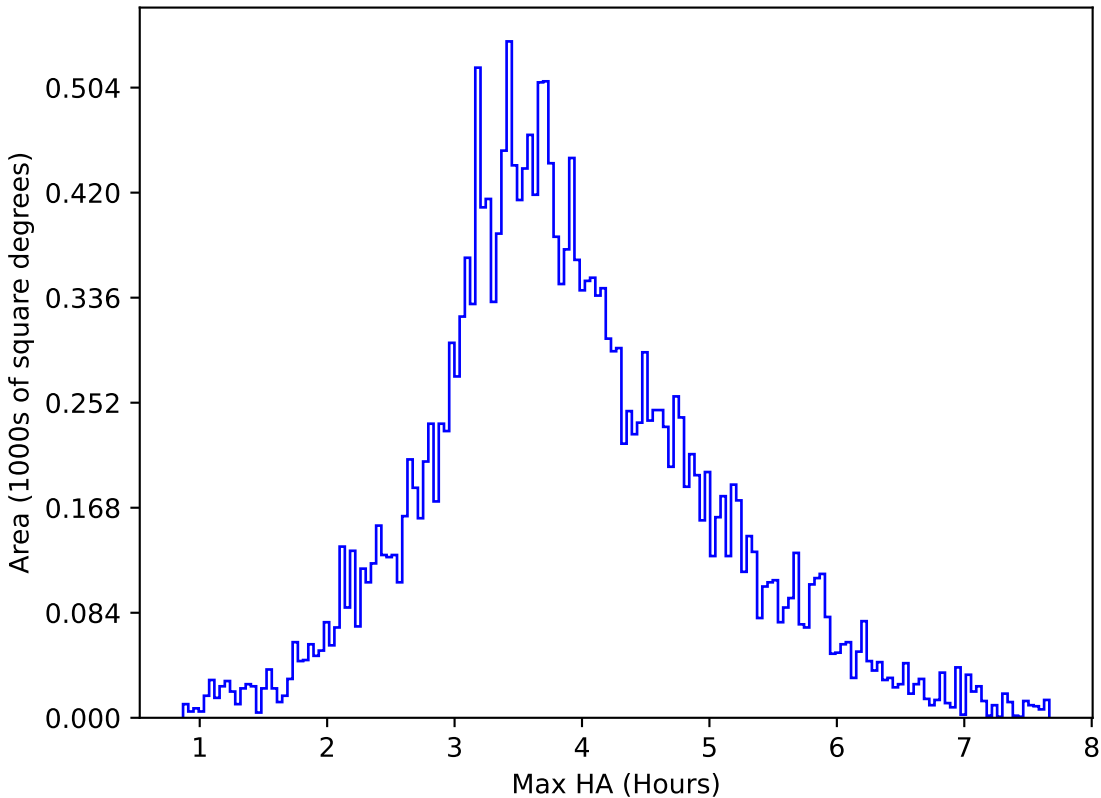
too_elab_heavy_r64_d3_gz_v3.4_10yrs All sky u band: Max HA
