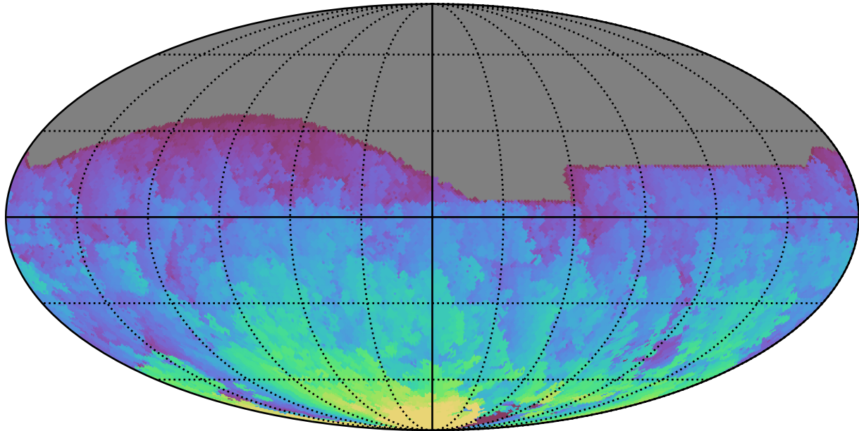
too_elab_heavy_r64_d3_gz_v3.4_10yrs All sky r band: Max HA
