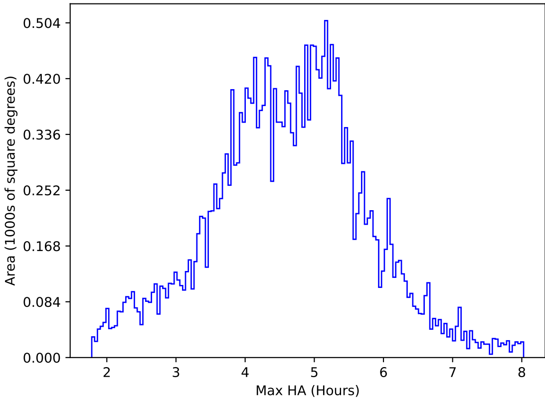
too_elab_heavy_r64_d3_gz_v3.4_10yrs All sky i band: Max HA
