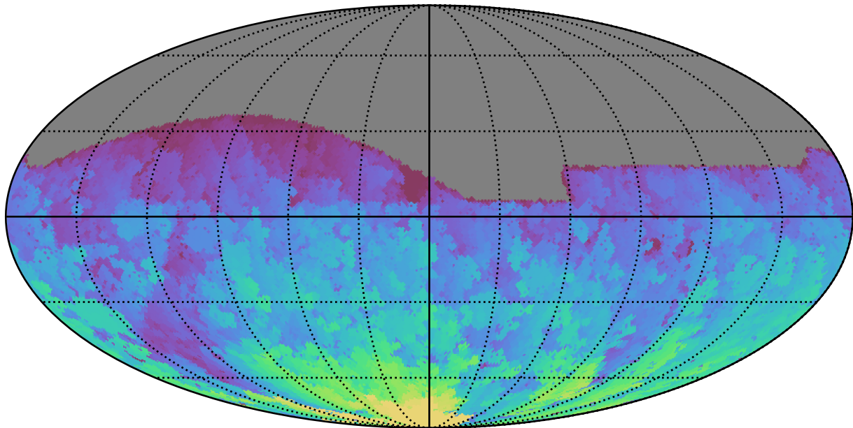
too_elab_heavy_r64_d3_gz_v3.4_10yrs All sky g band: Max HA
