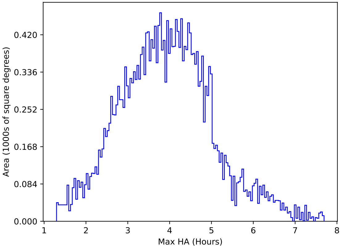
too_elab_heavy_r64_d3_gz_v3.4_10yrs All sky g band: Max HA
