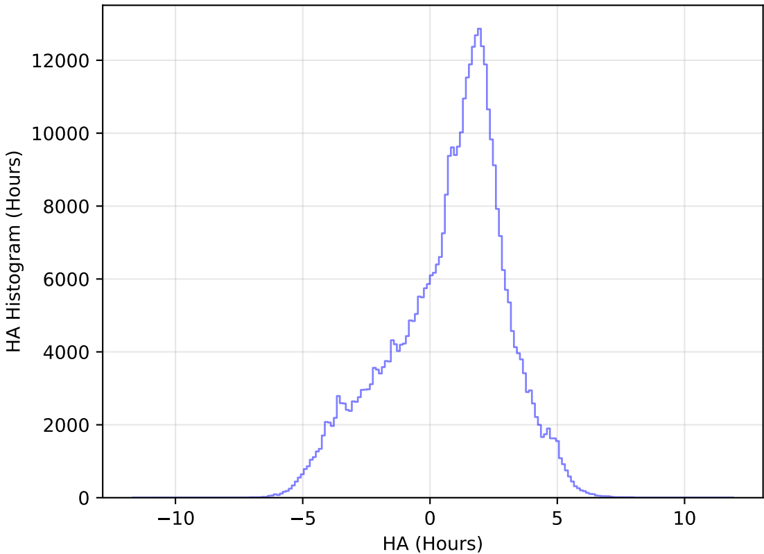
too_elab_heavy_r64_d3_gz_v3.4_10yrs WFD z band: HA Histogram
