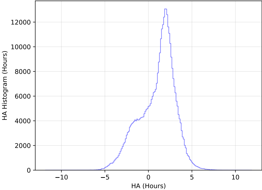
too_elab_heavy_r64_d3_gz_v3.4_10yrs WFD y band: HA Histogram
