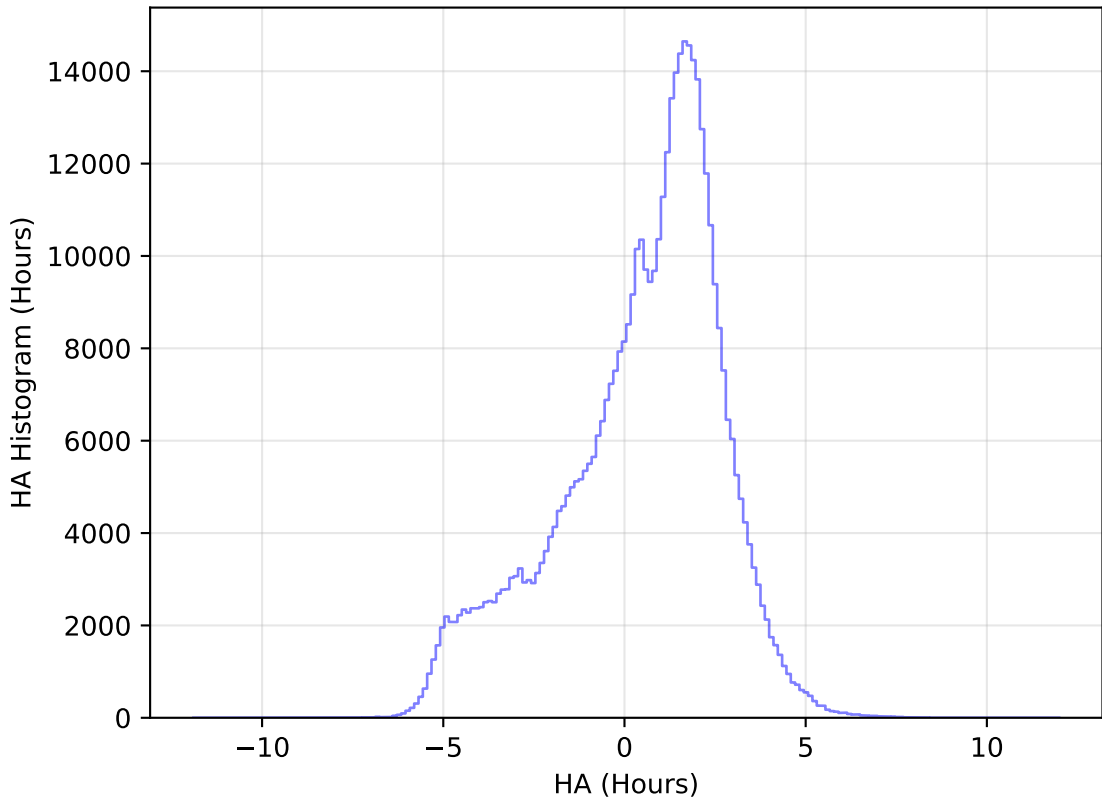
too_elab_heavy_r64_d3_gz_v3.4_10yrs WFD r band: HA Histogram
