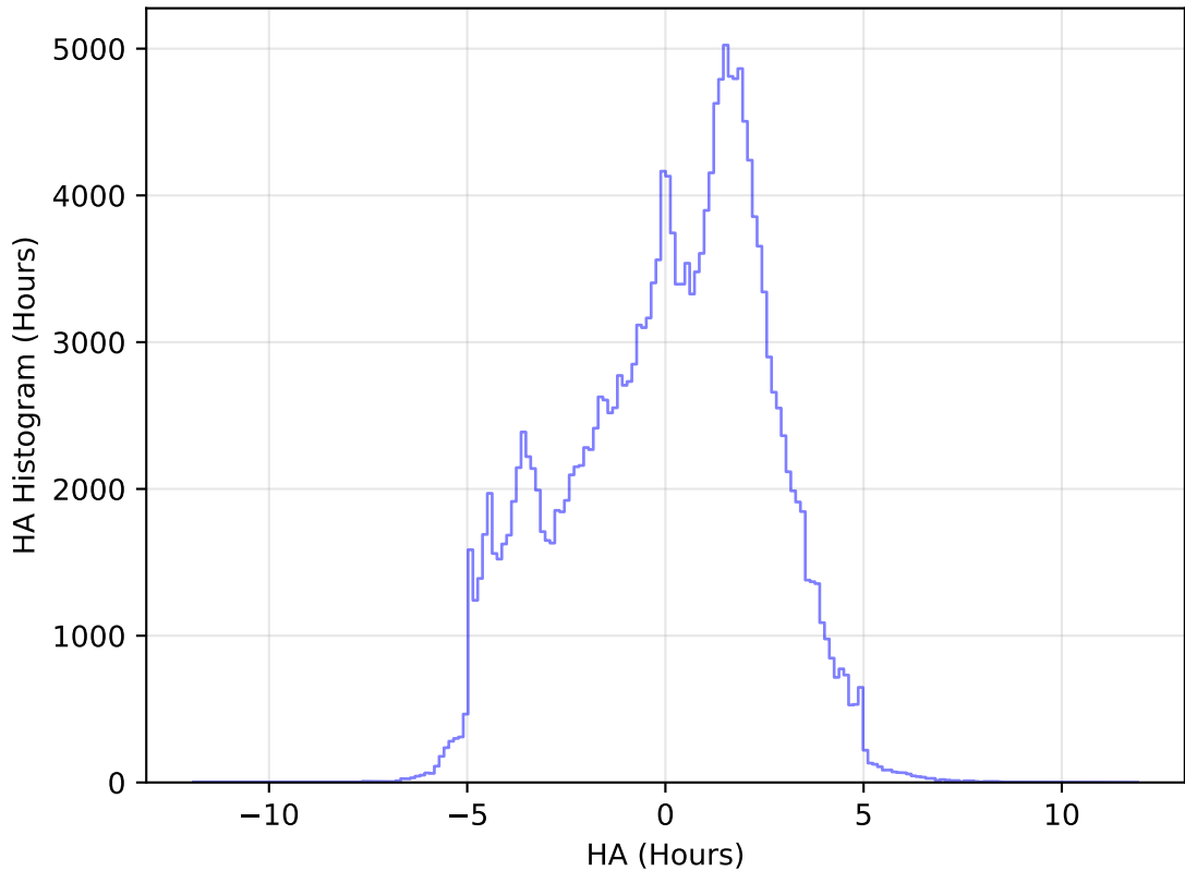
too_elab_heavy_r64_d3_gz_v3.4_10yrs WFD g band: HA Histogram
