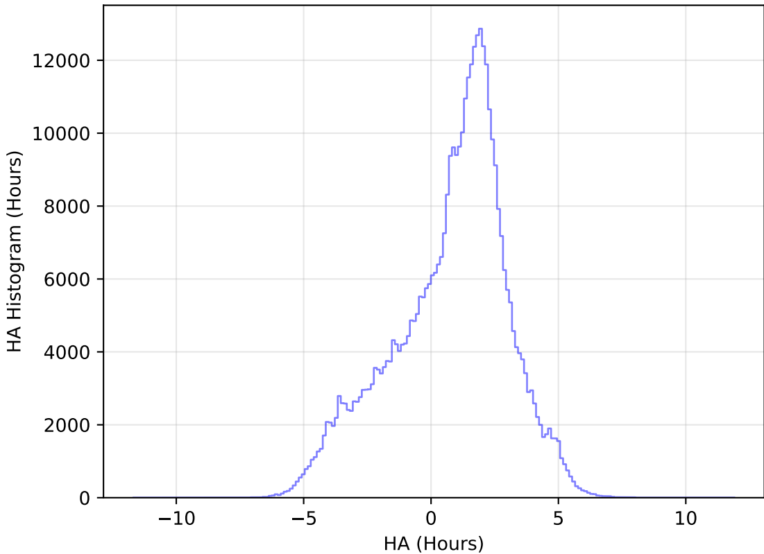
too_elab_heavy_r64_d3_gz_v3.4_10yrs All sky z band: HA Histogram
