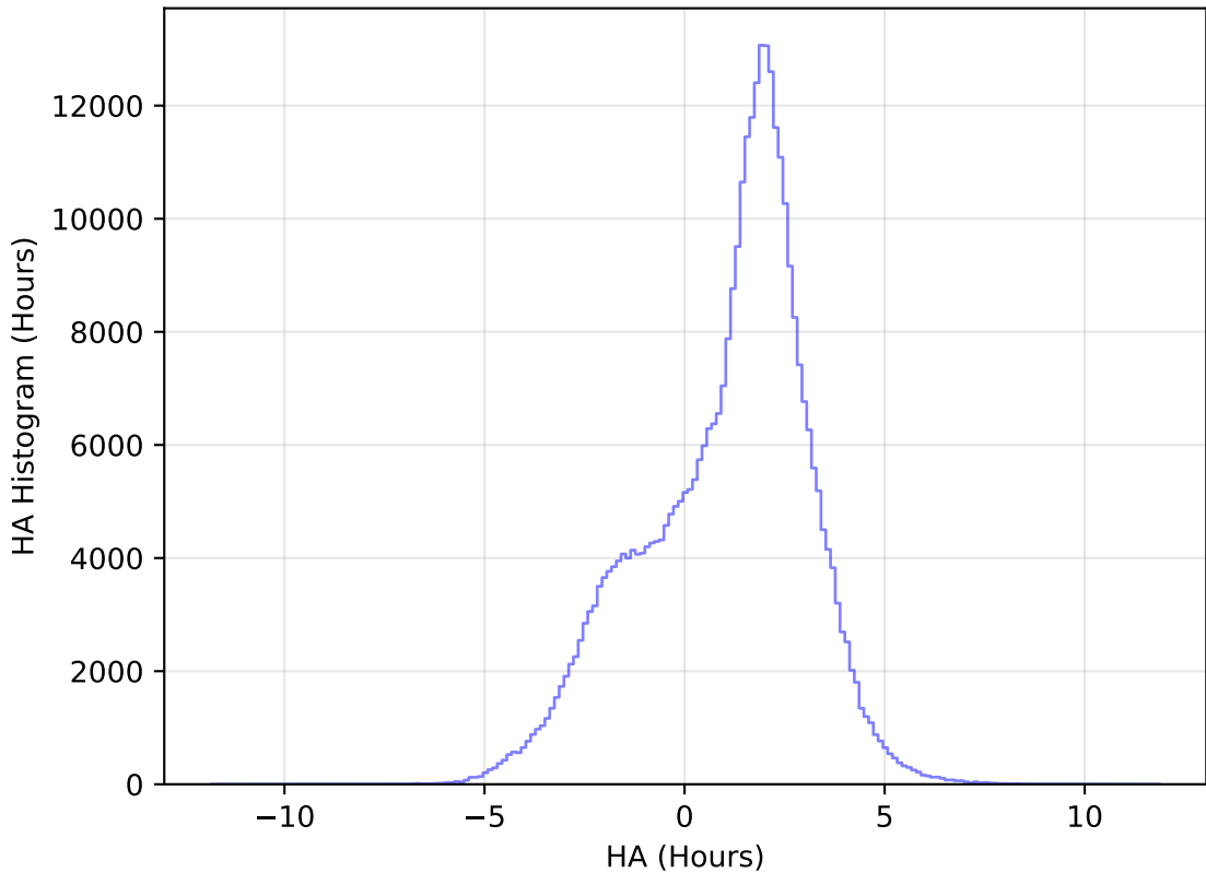
too_elab_heavy_r64_d3_gz_v3.4_10yrs All sky y band: HA Histogram
