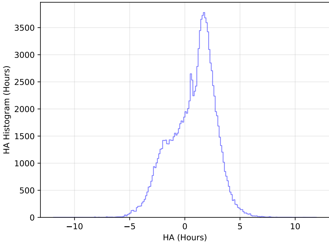
too_elab_heavy_r64_d3_gz_v3.4_10yrs All sky u band: HA Histogram
