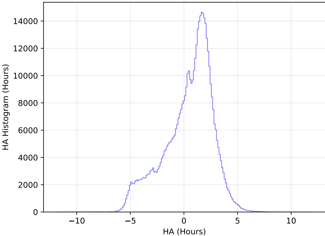
too_elab_heavy_r64_d3_gz_v3.4_10yrs All sky r band: HA Histogram
