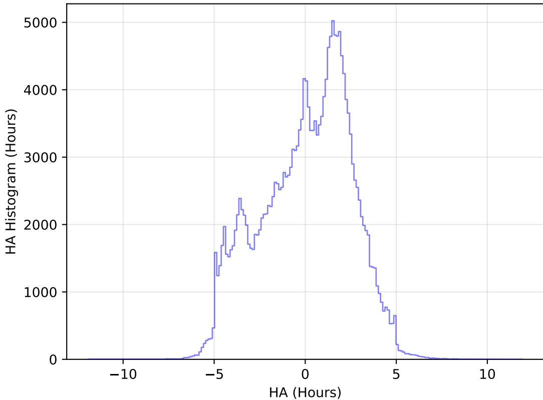
too_elab_heavy_r64_d3_gz_v3.4_10yrs All sky g band: HA Histogram
