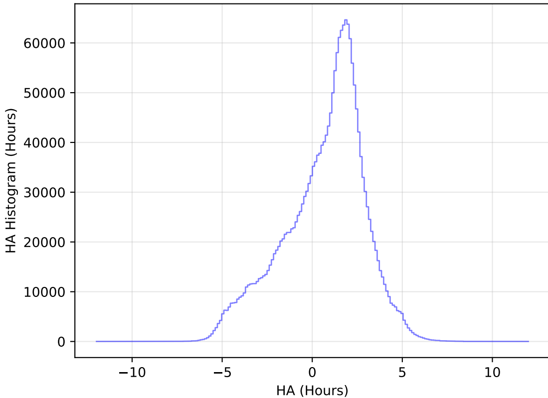
too_elab_heavy_r64_d3_gz_v3.4_10yrs All sky all bands: HA Histogram
