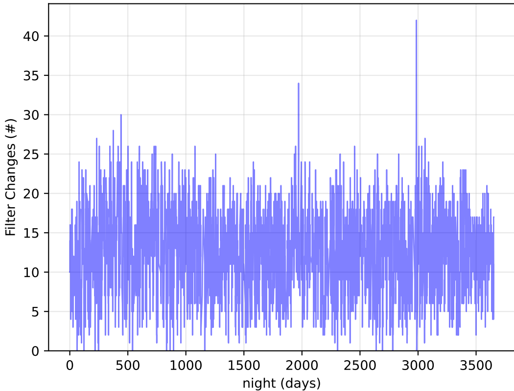
too_elab_heavy_r64_d3_gz_v3.4_10yrs Per Night: Filter Changes
