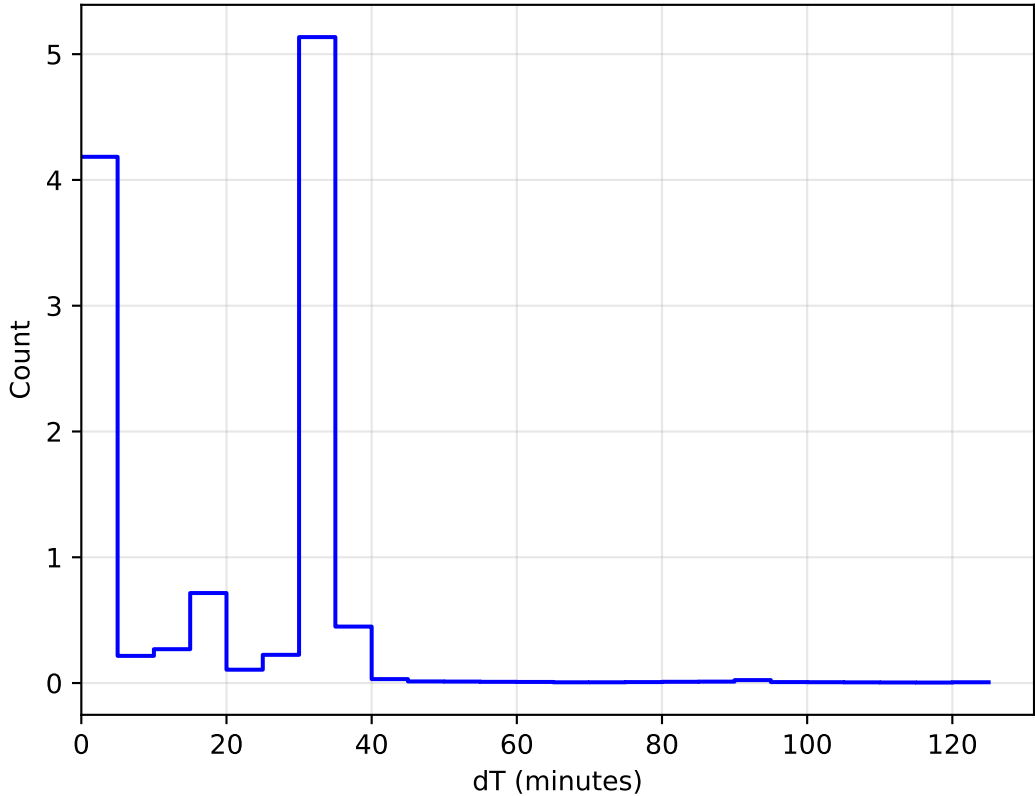
too_elab_heavy_r64_d3_gz_v3.4_10yrs WFD: DeltaT Histogram 1e6
