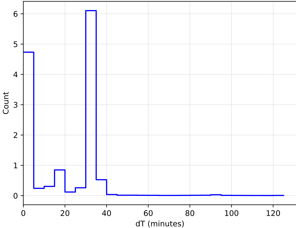
too_elab_heavy_r64_d3_gz_v3.4_10yrs All sky: DeltaT Histogram
