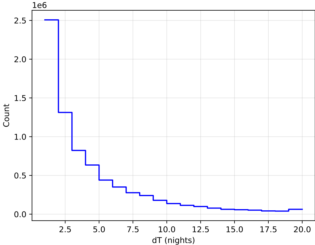
too_elab_heavy_r64_d3_gz_v3.4_10yrs WFD all bands: DeltaNight Histogram
