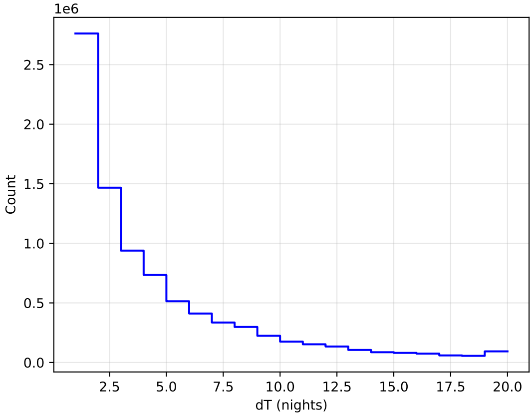
too_elab_heavy_r64_d3_gz_v3.4_10yrs All sky all bands: DeltaNight Histogram
