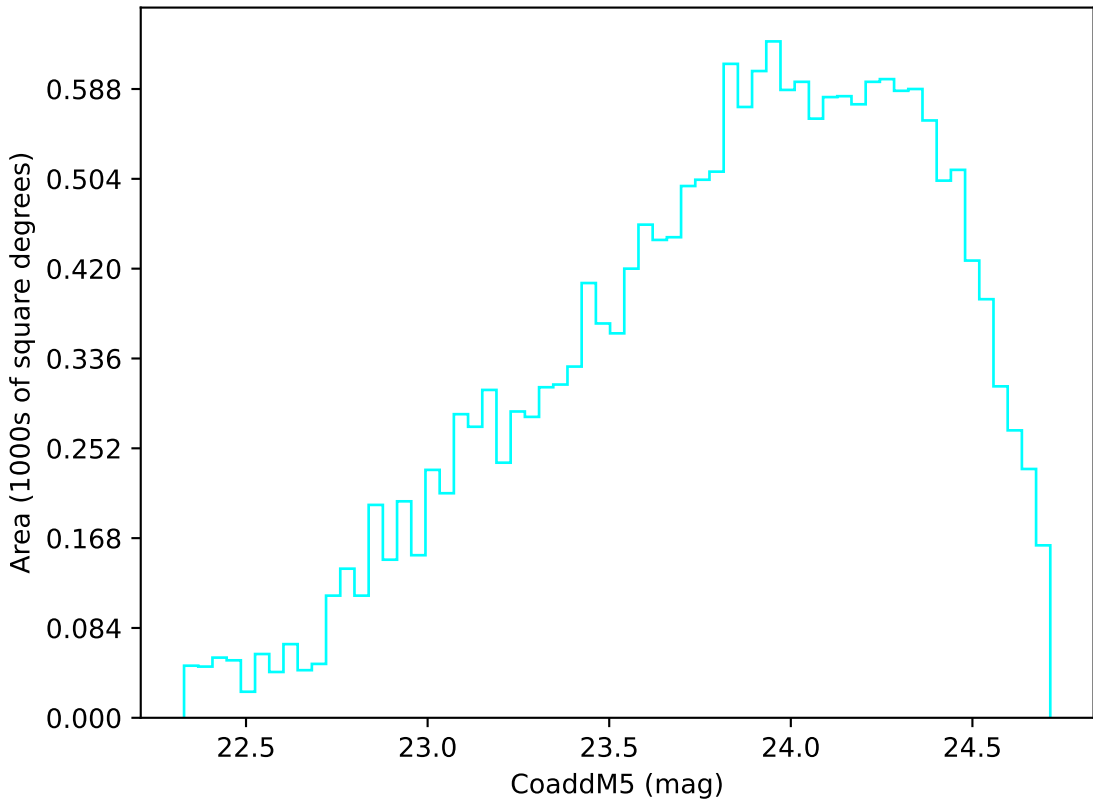
too_elab_heavy_r64_d3_gz_v3.4_10yrs Yr 3-4 u band: CoaddM5
