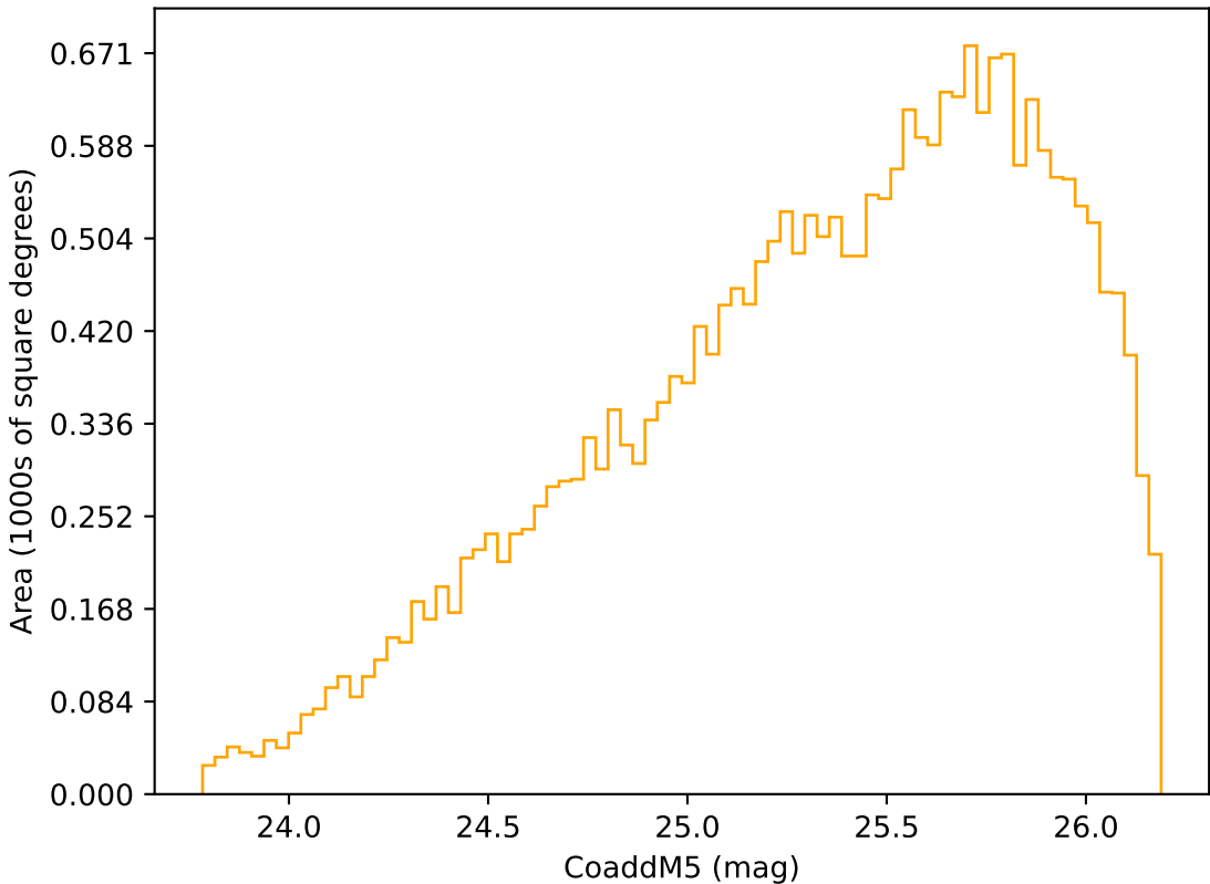
too_elab_heavy_r64_d3_gz_v3.4_10yrs Yr 3-4 r band: CoaddM5
