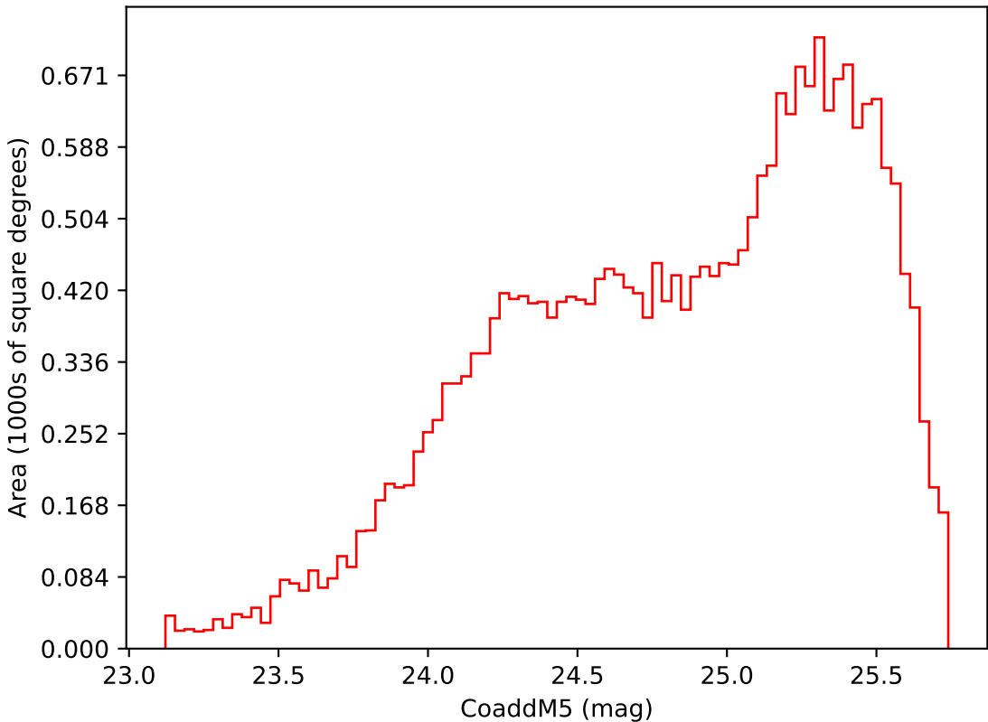
too_elab_heavy_r64_d3_gz_v3.4_10yrs Yr 3-4 i band: CoaddM5
