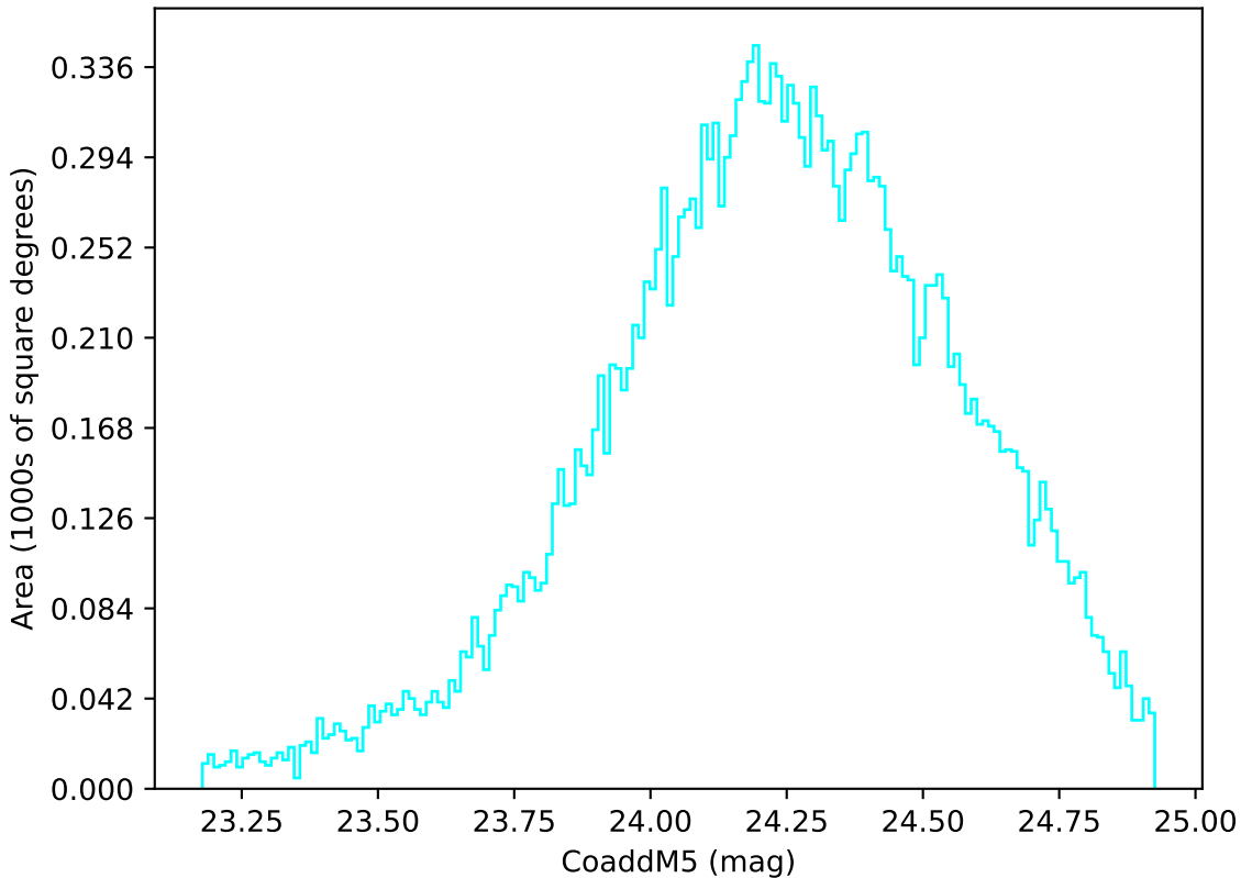
too_elab_heavy_r64_d3_gz_v3.4_10yrs Yr 1 u band: CoaddM5
