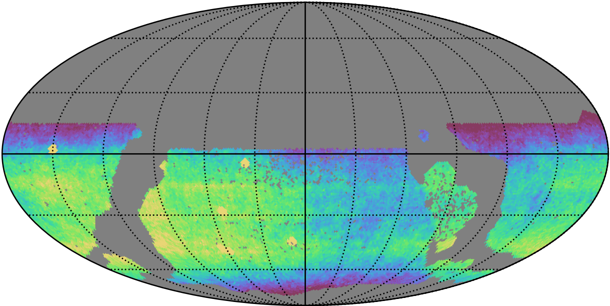
too_elab_heavy_r64_d3_gz_v3.4_10yrs WFD r band: CoaddM5
