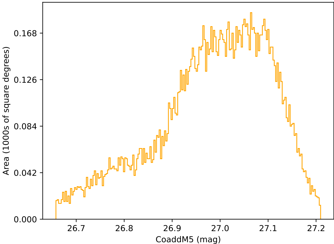
too_elab_heavy_r64_d3_gz_v3.4_10yrs WFD r band: CoaddM5
