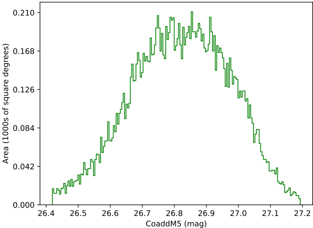
too_elab_heavy_r64_d3_gz_v3.4_10yrs WFD g band: CoaddM5
