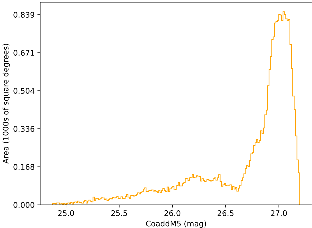
too_elab_heavy_r64_d3_gz_v3.4_10yrs All sky r band: CoaddM5
