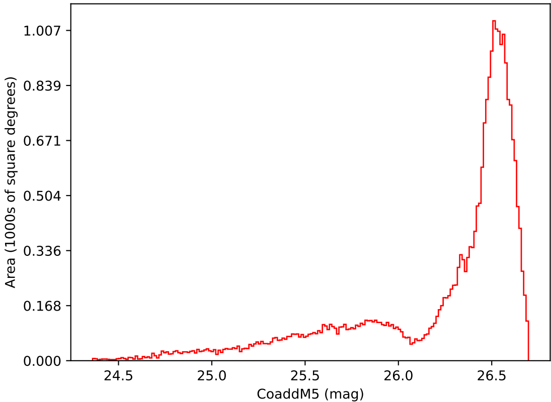
too_elab_heavy_r64_d3_gz_v3.4_10yrs All sky i band: CoaddM5
