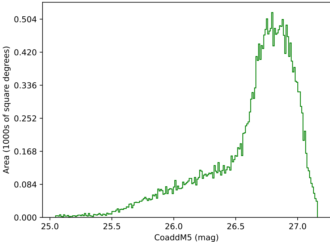
too_elab_heavy_r64_d3_gz_v3.4_10yrs All sky g band: CoaddM5
