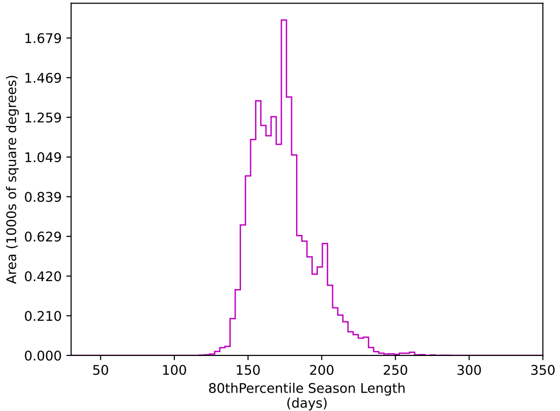
too_elab_heavy_r64_d3_gz_v3.4_10yrs WFD z band: 80thPercentile Season Length
