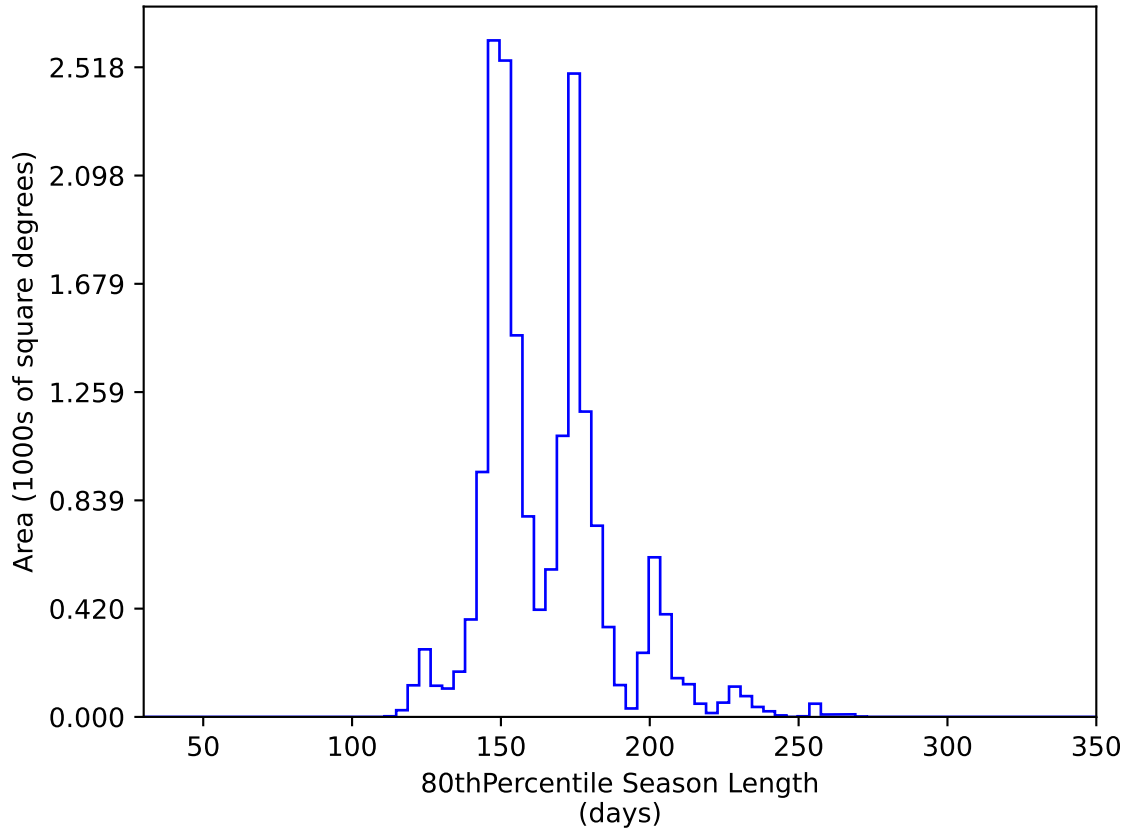
too_elab_heavy_r64_d3_gz_v3.4_10yrs WFD y band: 80thPercentile Season Length
